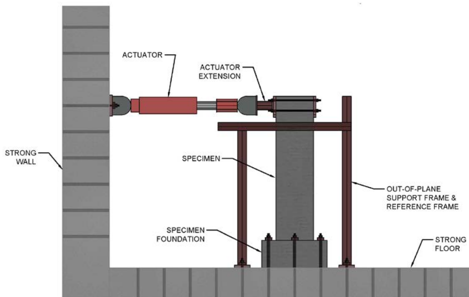
Fig.2 – Rendering of test set-up
