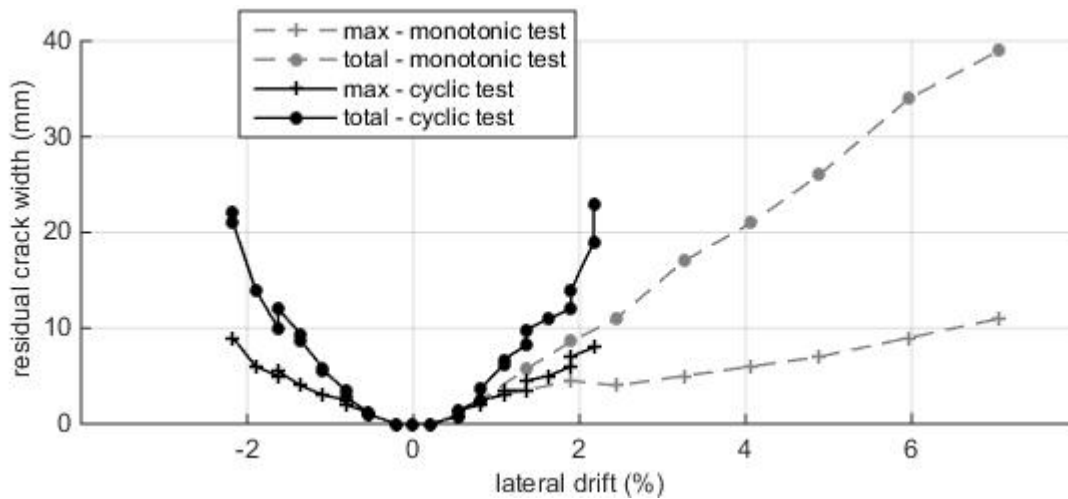
Fig. 6 – Residual crack widths (maximum and total) for specimen Cyc (black) and Mono (grey)
