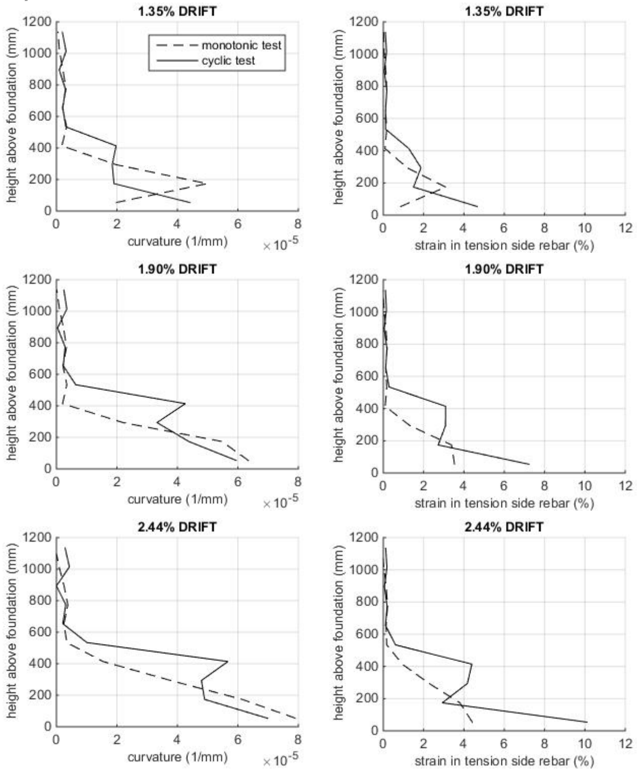
Fig.8 – Distribution of curvatures and strains in tension side reinforcement at increasing drift levels for specimen Cyc (solid line) and Mono (dashed line)
