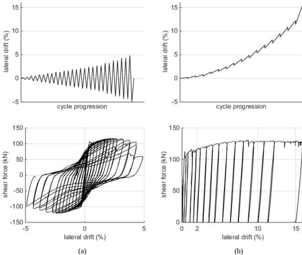
Fig.5 – Loading protocol and shear force vs lateral drift for specimen Cyc (a) and Mono (b)
