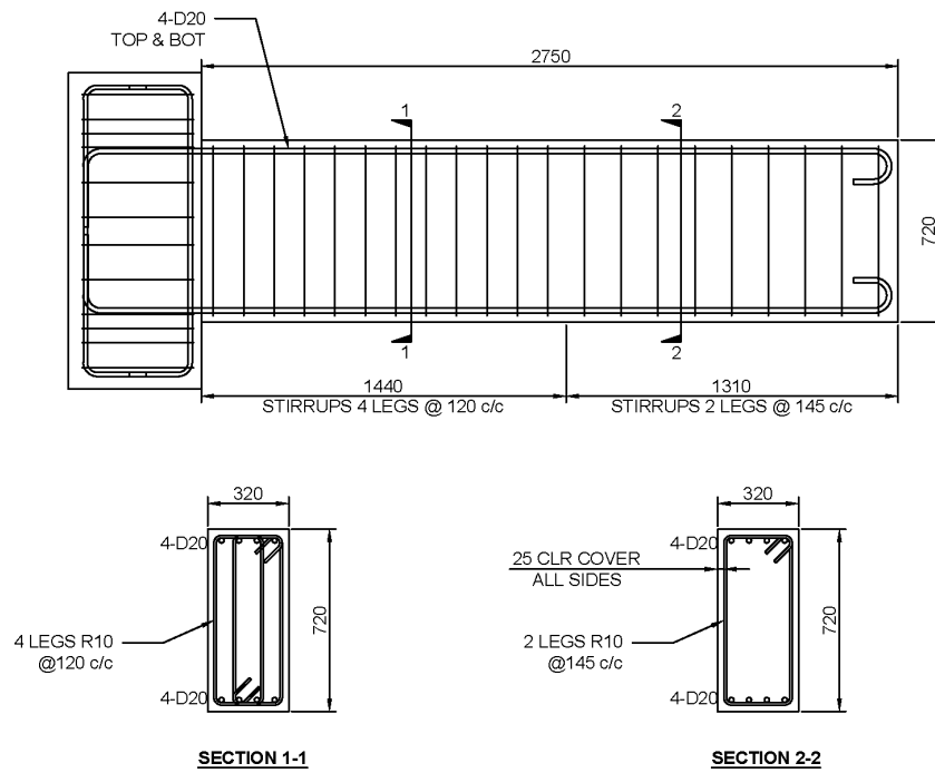
Fig.3 – Specimen detailing
