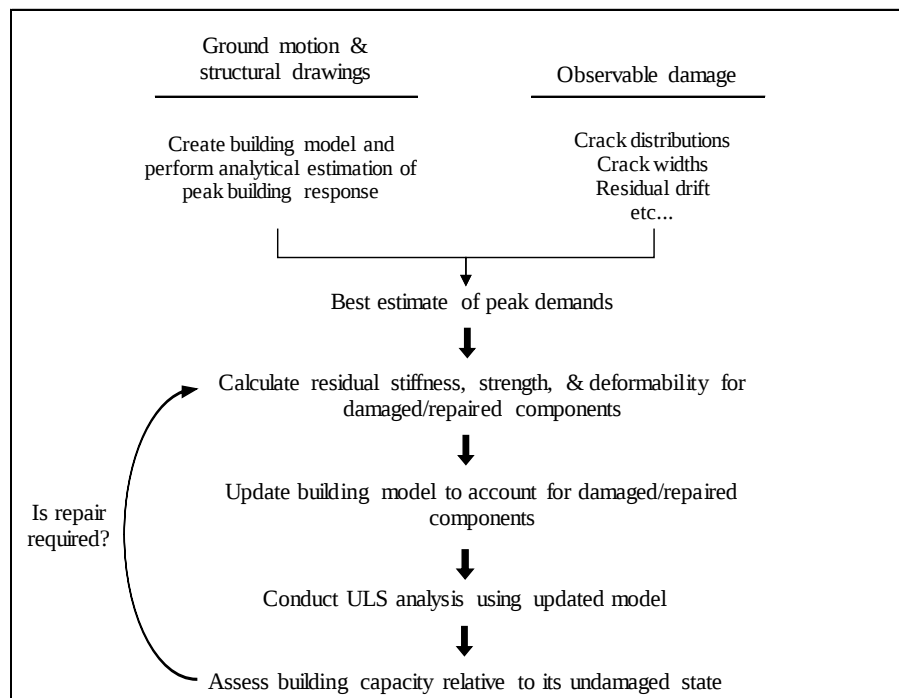
Fig.1 – Flowchart of proposed post-earthquake assessment methodology
