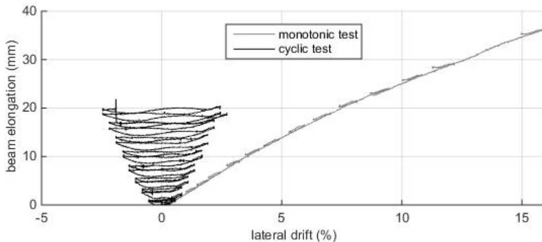
Fig.7 – Beam elongation for specimen Cyc (black line) and Mono (grey line)
