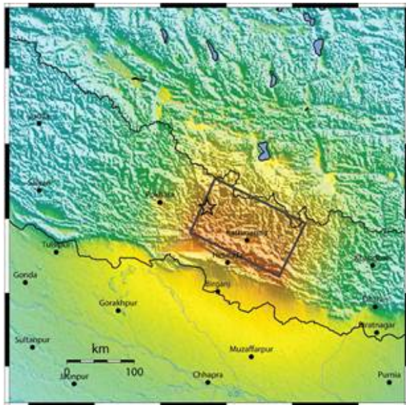
Fig. 4 USGS shakemap [1]
