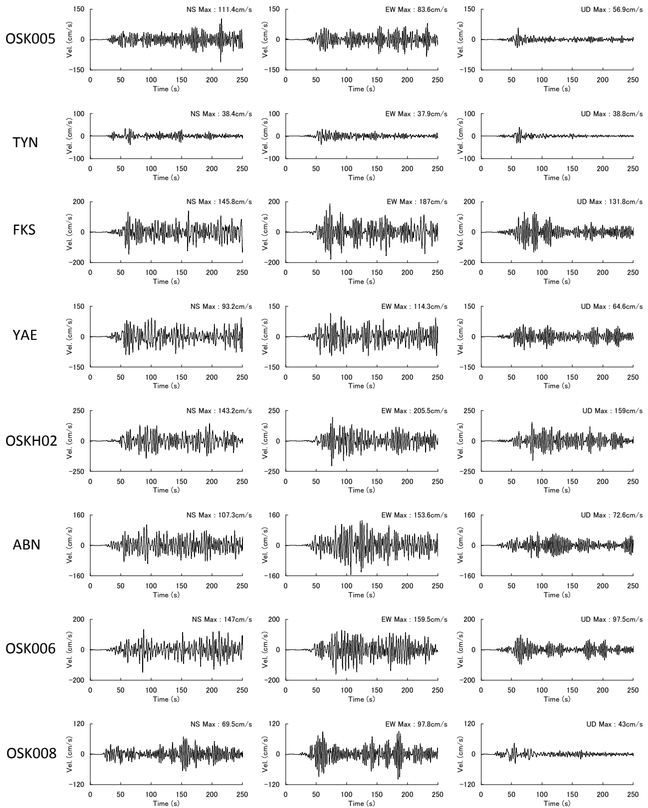
Fig. 5 – Synthesized velocity ground motion (0.05–0.4 Hz).
