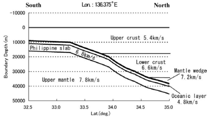
Fig. 1 – North–south cross-section of the crustal velocity structure model at longitude 136.375°E.
