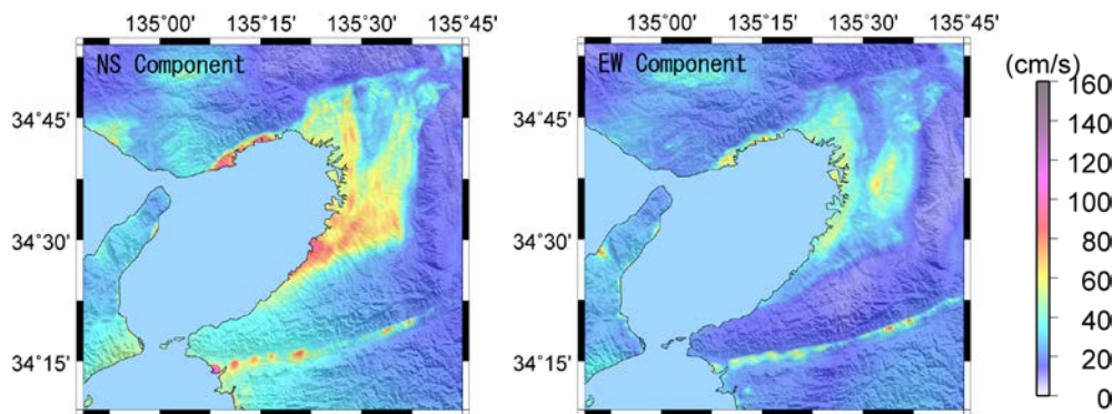
Fig. 4 – Simulated peak ground velocity distribution for the Nankai earthquake in the Osaka basin (0.05–0.4 Hz).
