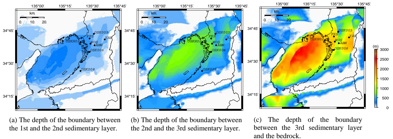
Fig. 2 – Topography of the bedrock surface and the boundaries between sedimentary layers of the Osaka sedimentary basin structure model.
