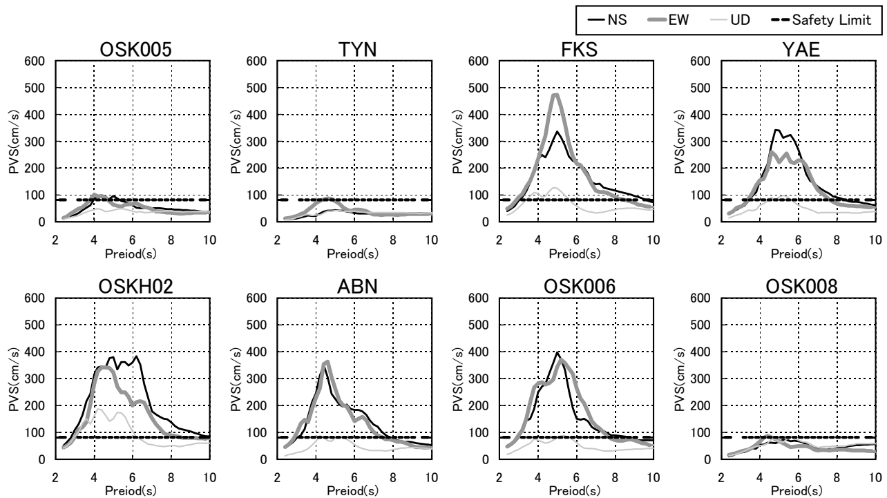
Fig. 7 – Pseudo velocity response spectra with 5% damping ratio and the safety limit level of the building design criterion in Japan. The safety limit level is defined for horizontal components at the engineering bedrock surface.
