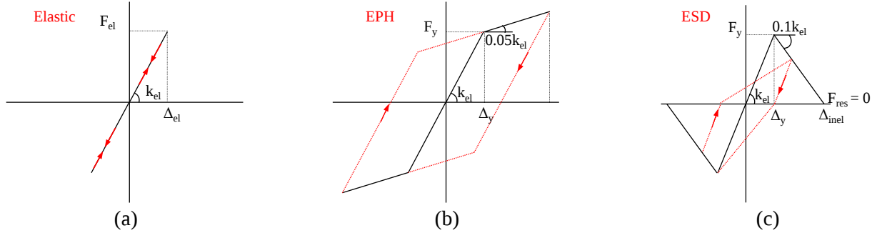
Figure 4 - SDOF systems analysed (a) Linear Elastic, (b) EPH (c) ESD [adapted from [38]].
