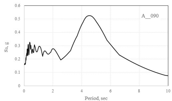
Fig. 2 5%-damped response spectrum, 90-degree component
