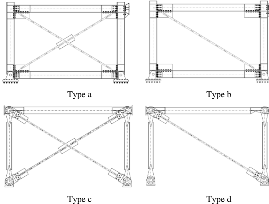
Fig. 11 Test specimens designed to investigate the contribution of compression diagonal
