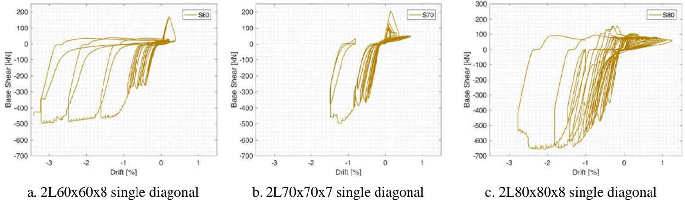
Fig. 14 Global base shear-drift behaviour of single diagonal specimens tested until global collapse
