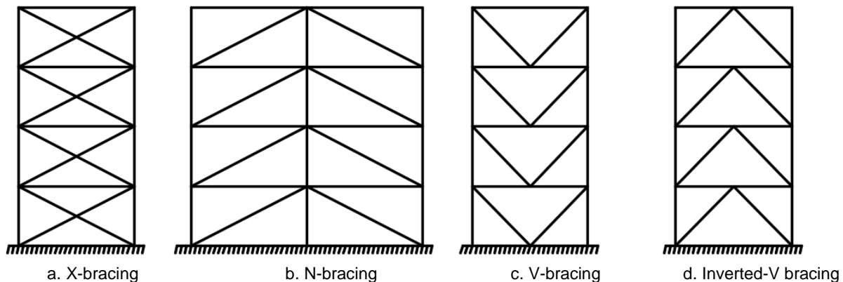
Fig. 1 Concentrically braced frame configurations classified by Eurocode 8.
