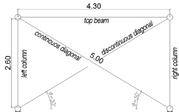
b. Frame with ideally pinned joints
