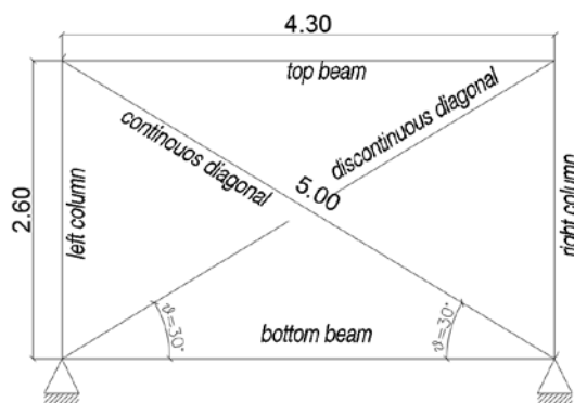
a. Frame with semi-rigid joints
