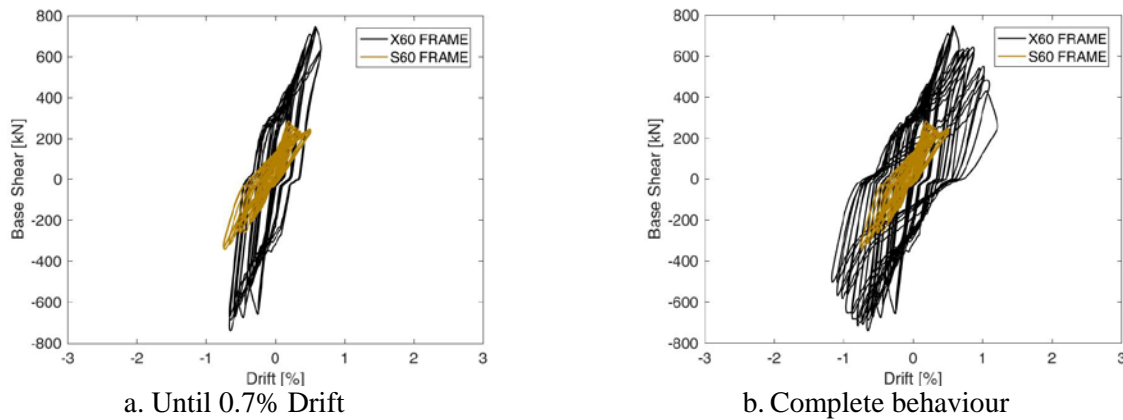
Fig. 13 Contribution of compression diagonal on global behaviour for X-braced specimen 2L60x60x8
