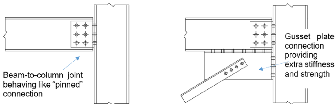
a. Beam-to-column connection without gusset plate b. Beam-to-column connection with gusset plate Fig. 7 Beam-to-column connections with and without bracing gusset plate
