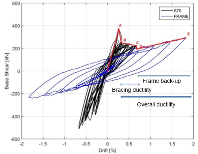
b. 2L70x70x7 single diagonal
