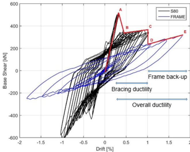
c. 2L80x80x8 single diagonal
