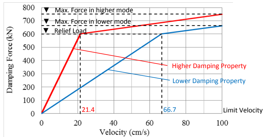
Fig. 7 – Damping Property of Passive-Switching Oil Damper
