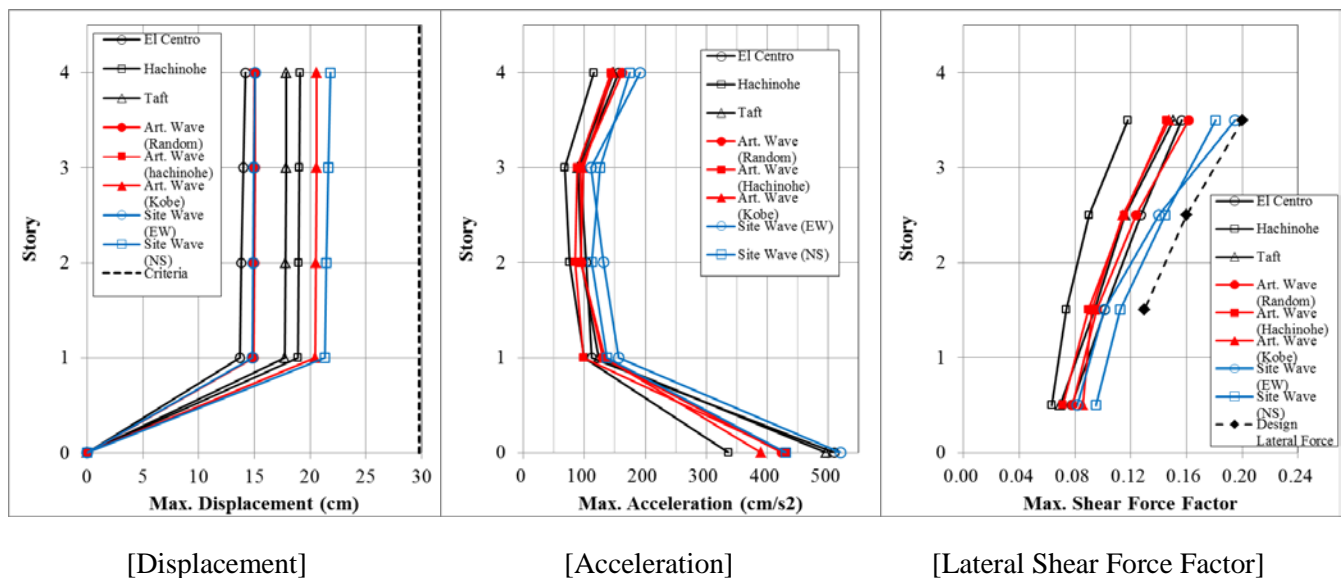
Fig. 8 – Maximum Response Values (major earthquakes)
