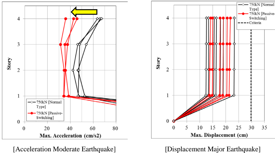
Fig. 9 – Comparison of Maximum Response Values between Passive-Switching Oil Damper and Conventional Oil Damper
