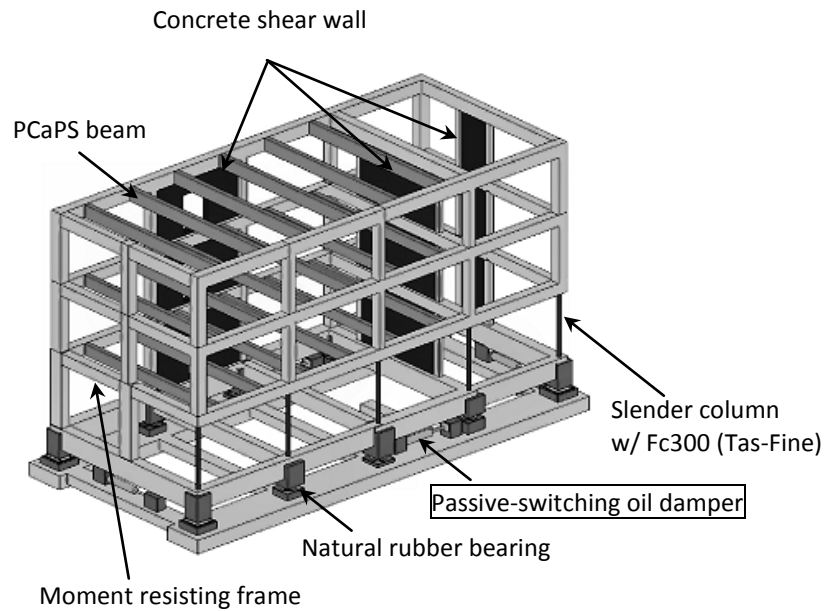
Fig. 5 – Structural System of Superstructure
