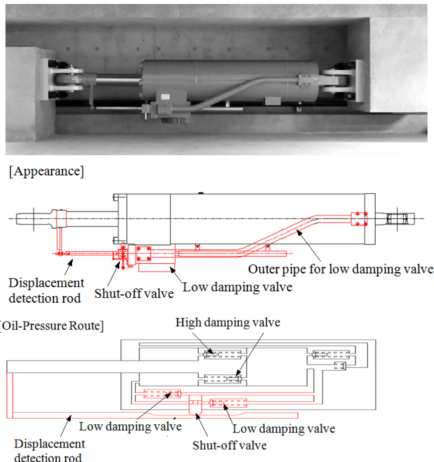
Fig. 2 – Appearance and Oil-Pressure Route of Passive-Switching Oil Damper
