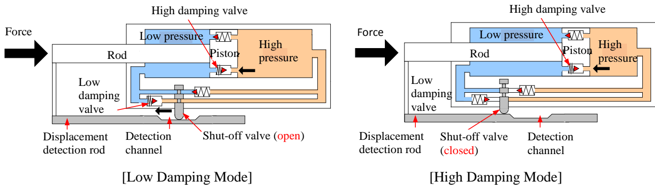
Fig. 3 – Mechanical Principle of Passive-Switching Oil Damper
