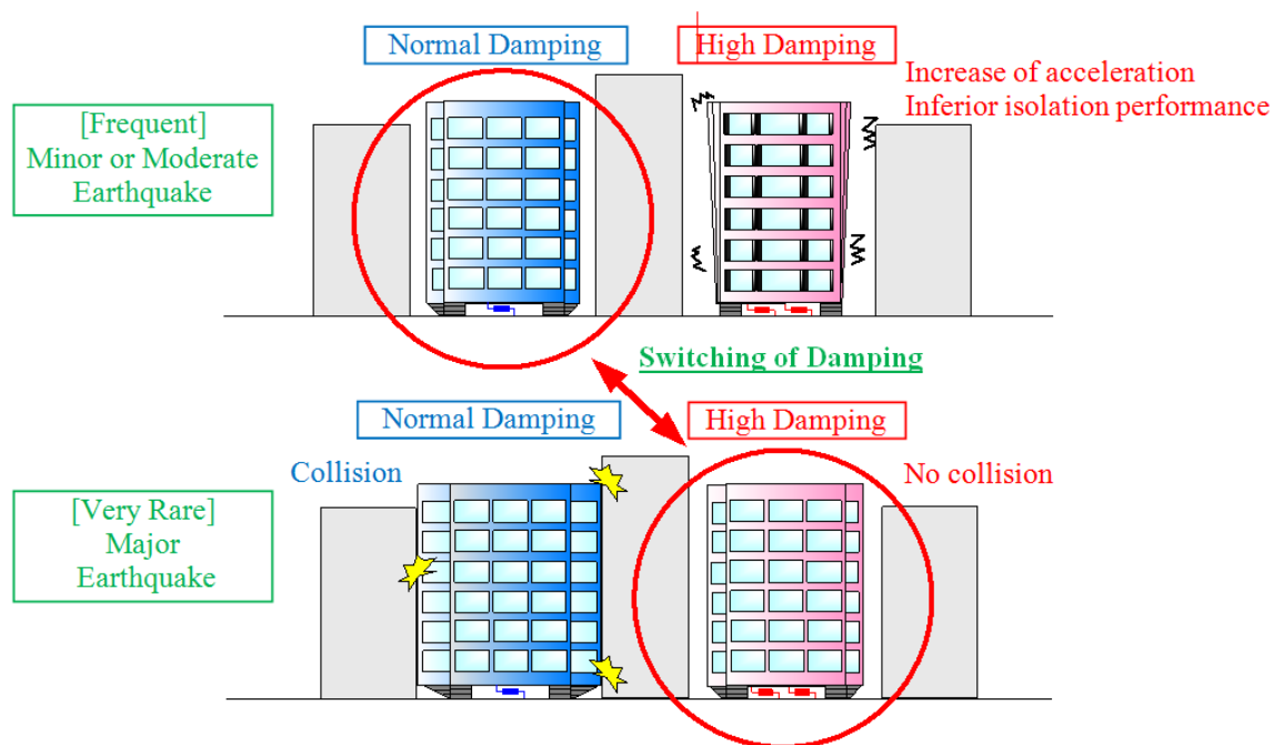
Fig. 1 – Principle of Short Stroke Seismic Isolated System with passive-switching oil damper
