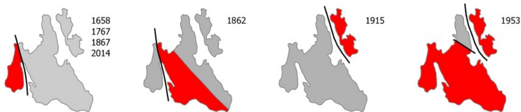
Fig. 7 – Areas with high contrasts in seismic intensities during major earthquakes in Cephalonia. The highest intensities have undoubtedly been observed in the Paliki peninsula (IX-X MMI during the 1658, 1767, 1867, 1953 and 2014 earthquakes). On the contrary, the Erissos peninsula is the only macrostructure that suffered low intensities (IV-VI MMI during the 1658, 1767, 1862, 1867, 1915, 1953 and 2014 earthquakes) [31, this study].
