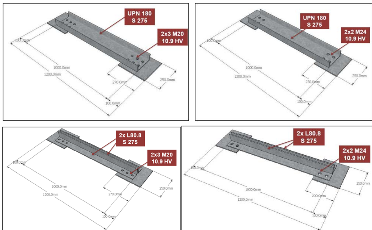
Fig. 2 – Test specimens
