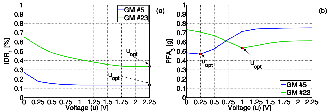
Fig. 5 - Example of EDPs vs voltage curves and optimal voltage values for two generic ground motion records: (a) IDR at the first story; (b) PFA at the third story.
