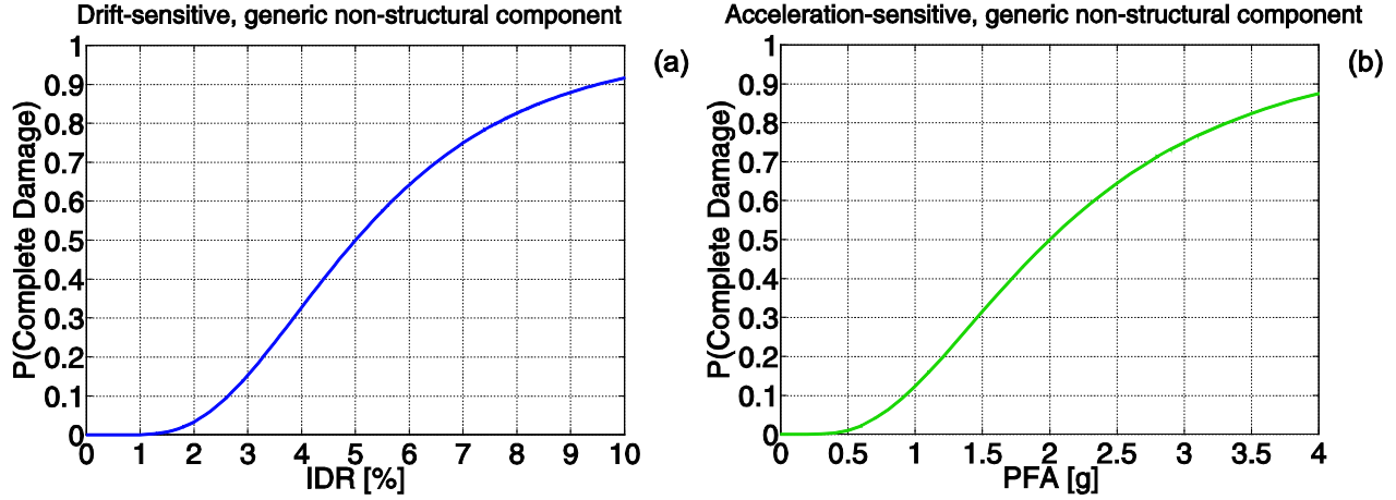
Fig. 6 - Fragility functions for complete damage for (a) drift-sensitive, generic non-structural component (in office buildings); and (b) acceleration-sensitive, generic non-structural component (in office buildings).
