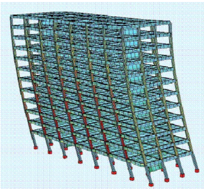
Fig. 7 - Model Building – First mode shape
