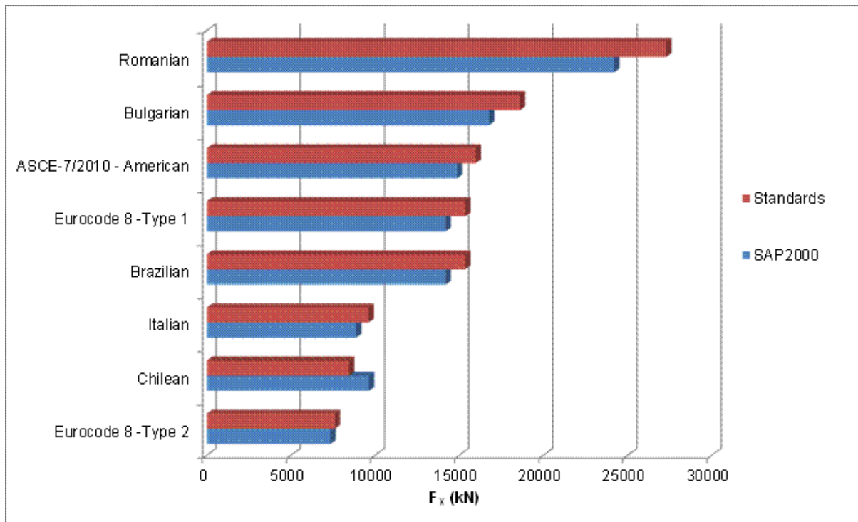
Fig.11 – Base shear at the longitudinal direction X
