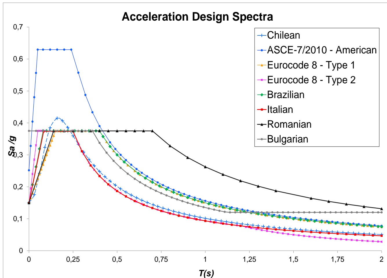
Fig. 2 - Elastic response spectra for the analyzed building according to the standards
