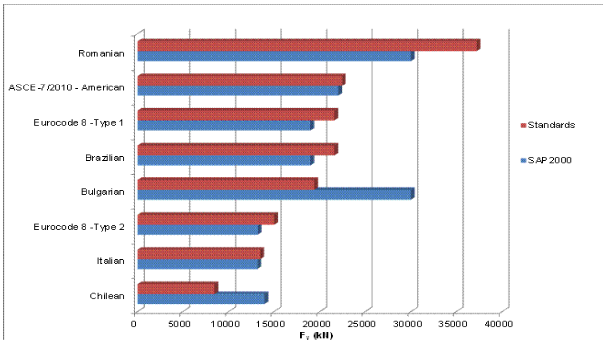
Fig.12 - Base shear at the transversal direction Y
