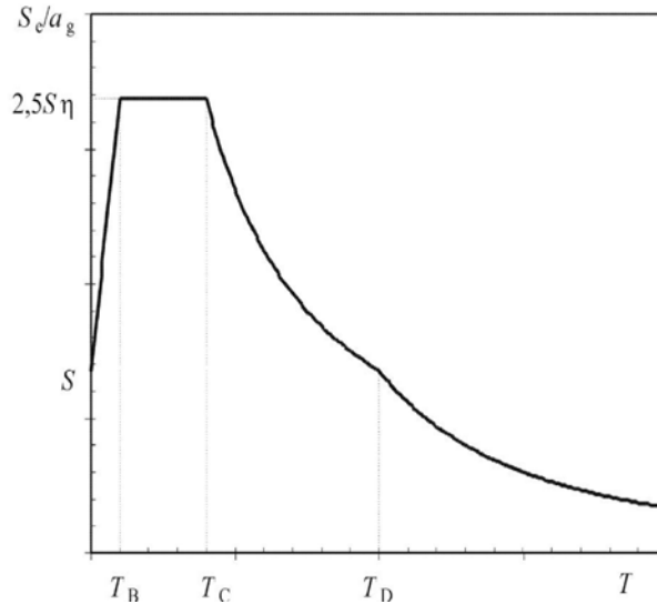
Fig. 1 –Shape of the elastic response spectrum
