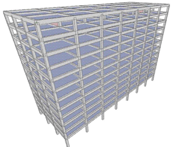
Fig. 6 - Perspective generated by SAP2000
