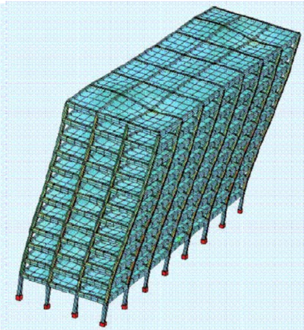
Fig. 8 - Model Building – Second mode shape
