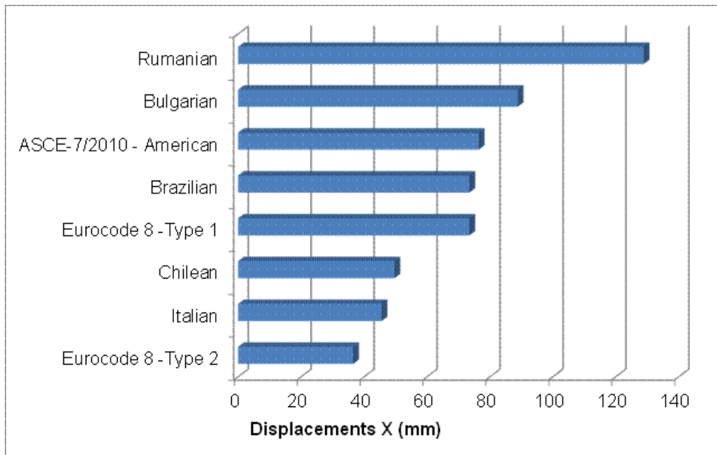
Fig. 9 – Displacements at the top, at the longitudinal direction X
