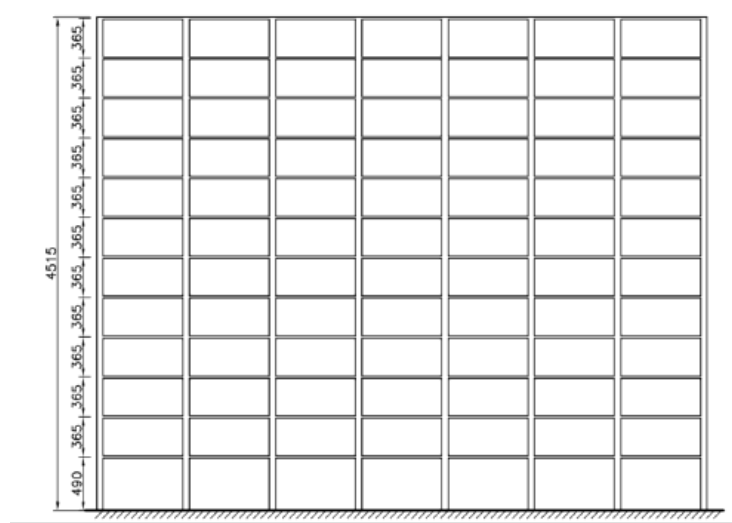
Fig. 4 - Model Building - Longitudinal section
