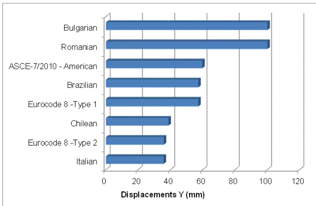
Fig. 10 – Displacements at the top, at the transversal direction Y
