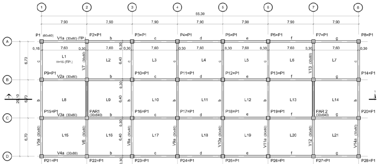
Fig. 3 – Model Building – Formwork - Typical floor plan
